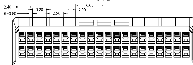
40PIN-X
