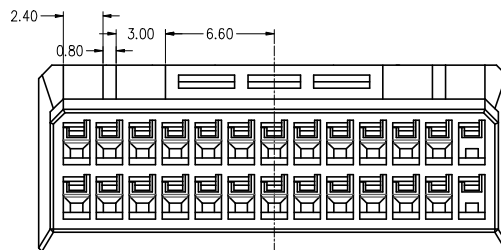
26PIN-X
