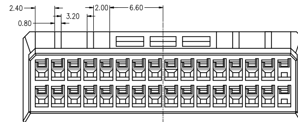
32PIN-X
