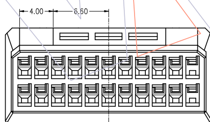
22PIN-X
