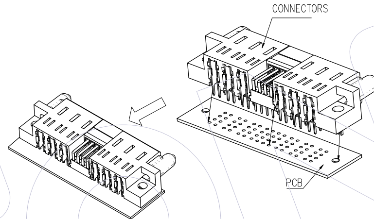
△3 PSP 90°DIP INSTALL CONNECTORS PCB
