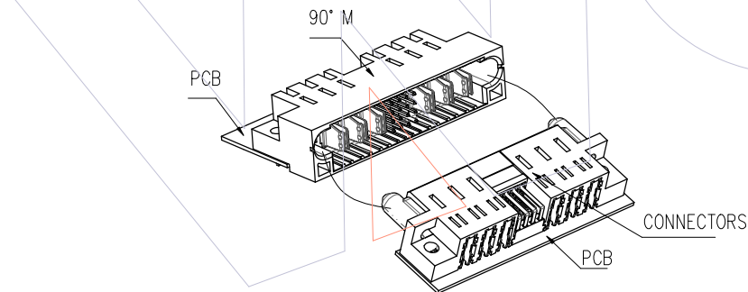
△3 Attempt to Match with 90° M
