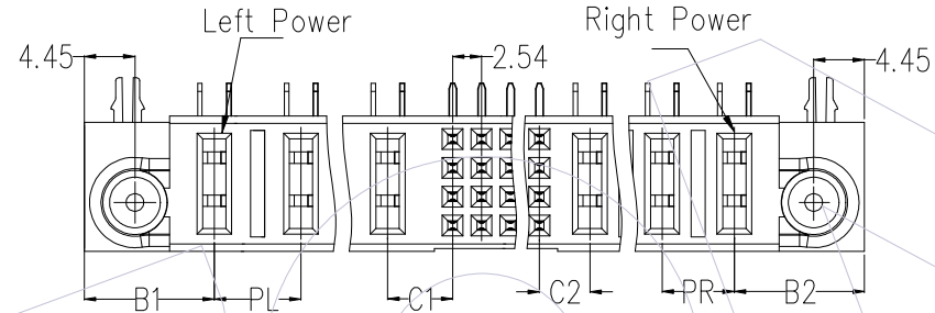
△3 Schematic diagram of terminal spacing
