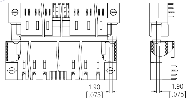
△3 Blind Mate Guide Ends SCALE: 1:2
