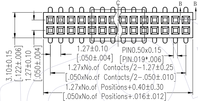
Special CAP for 2*2P, 2*3P, 2*4P
